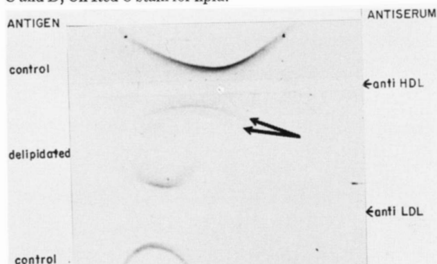
Fig. 4. Immunoelectrophoresis of control and delipidated whole serum lipoproteins on agarose gel. Antibody troughs contained antisera to human HDL or LDL. Antigen wells contained whole control serum or delipidated whole serum. The arrows indicate the two arcs present only when lipoproteins from delipidated serum reacted against anti-HDL. Migration was from left to right. Proteins were stained with Coomassie Blue.
