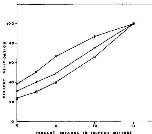
Fig. 2. Extraction of total, unesterified- and esterified cholesterol in 1 hr by butanol-DIPE mixtures; X, total cholesterol; \nabla , unesterified cholesterol; \square , esterified cholesterol. Control values (mg per 100 ml of plasma) were: total cholesterol, 205; unesterified cholesterol, 69; and esterified cholesterol, 136.
