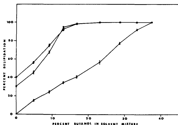
Fig. 1. Delipidation of human plasma in 1 hr by butanol-DIPE mixtures; O, triglyceride; X, cholesterol; \Delta , phospholipid. Values are means \pm SD of five estimations. Range of initial concentrations (mg per 100 ml of plasma) were: triglyceride, 100-233; cholesterol, 187-290; phospholipid, 180-270.
