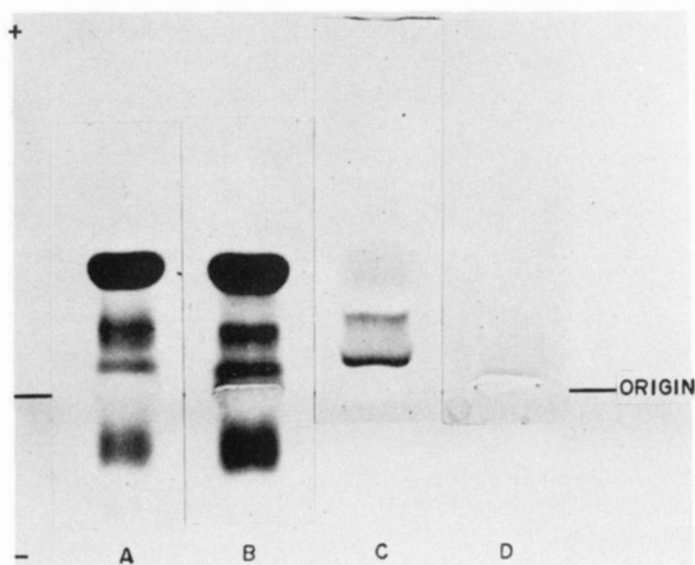
Fig. 3. Electrophoretic strips comparing control (unextracted) human plasma with human plasma extracted with butanol-DIPE 40:60 (v/v) for 0.5 hr. A and D, delipidated plasma; B and C control plasma; A and B, Coomassie Blue stain for protein; C and D, Oil Red O stain for lipid.
